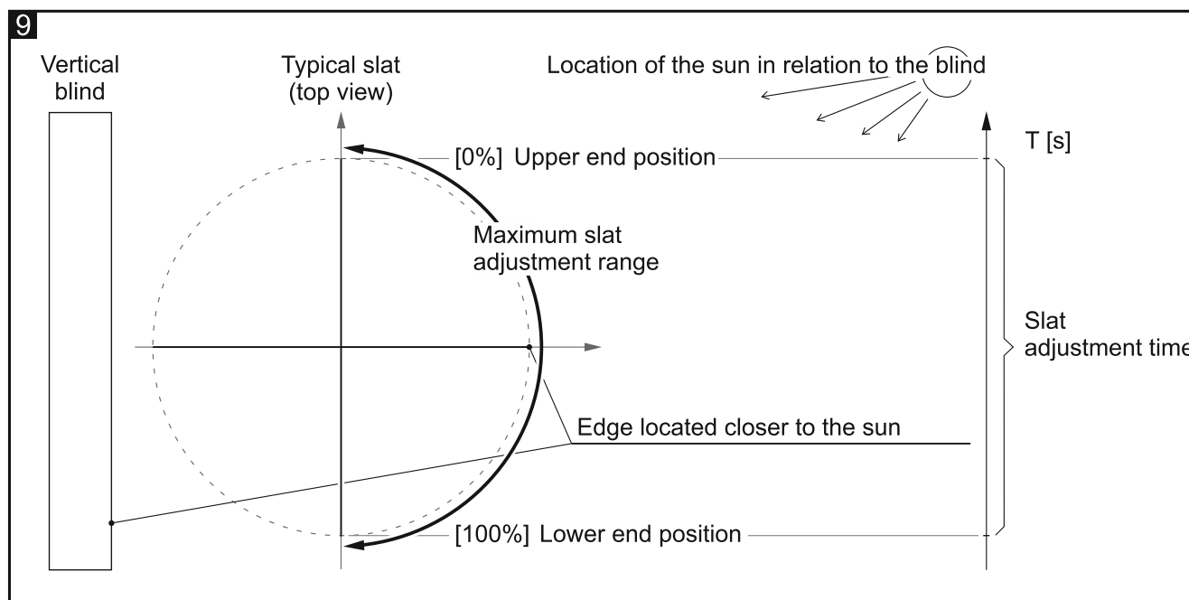
Fig. 9 shows how to define the slat position and adjustment time for a vertical blind (only for the KNX-BSA12L module).
